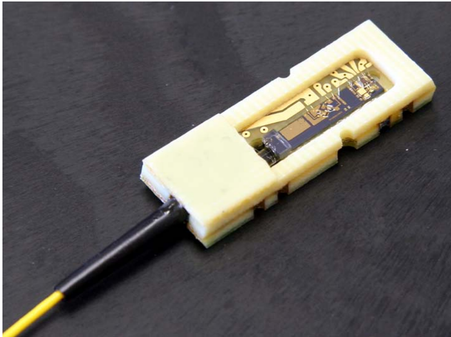
Figure 2 | A compact, lightweight, bidirectional optical transceiver that can transmit and receive simultaneously at 2.5 Gbps, while also receiving analog video signals at up to 1 GHz on a third channel.
